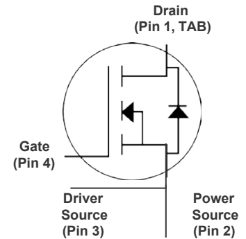
TO-247H-4L (TO-247H-4)
