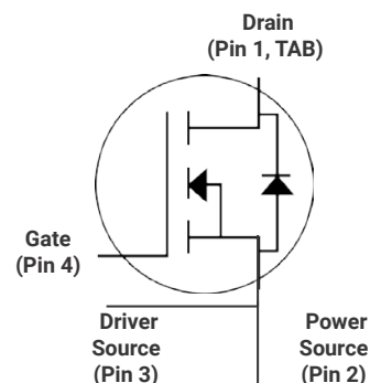
TO-247H-4L
