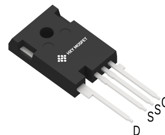
TO-247H-4L
