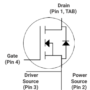
TO-247H-4L
