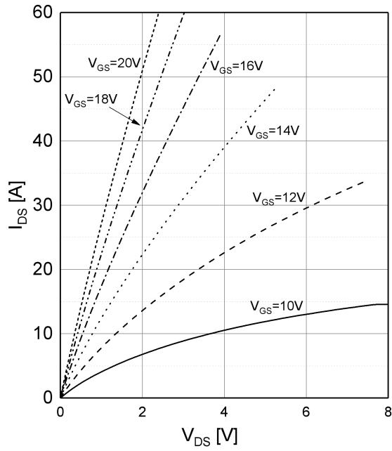
Output characteristics I_{DS}=f(V_{DS}) , T_J=150^{\circ}\text{C}
