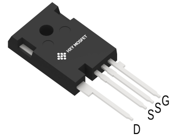
TO-247H-4L (TO-247H-4)
