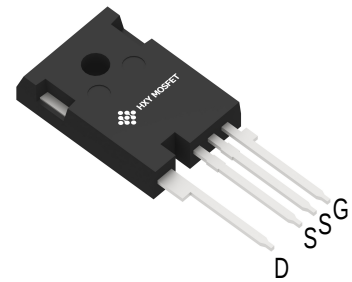
TO-247H-4L
