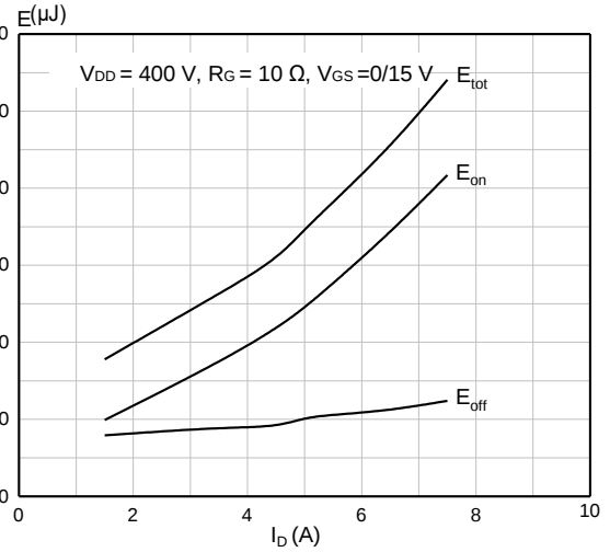
Figure 10. Typical Switching Energy vs. Drain Current
