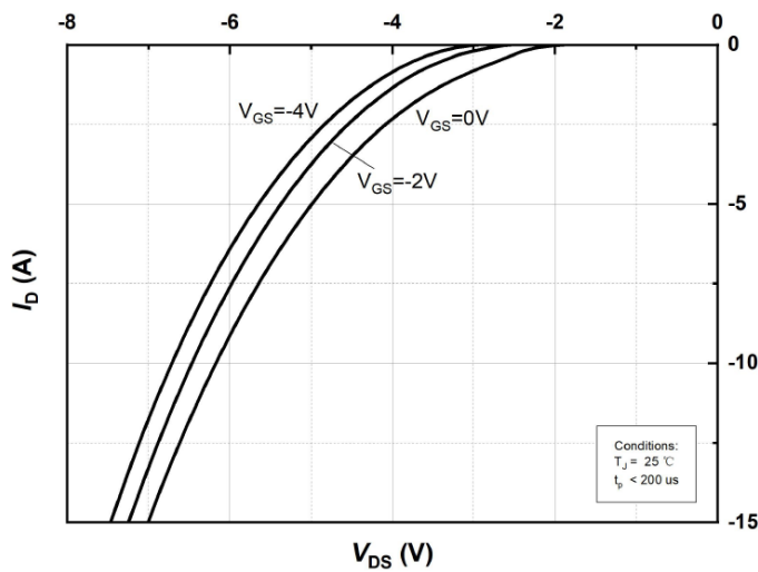
Figure 7. Body Diode Characteristics at T J =25°C
