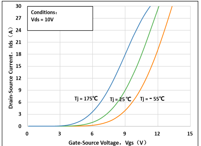
Fig 6: Transfer Characteristic
