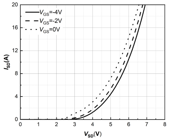
Figure 8. Body Diode Characteristic T_J = -40°C
