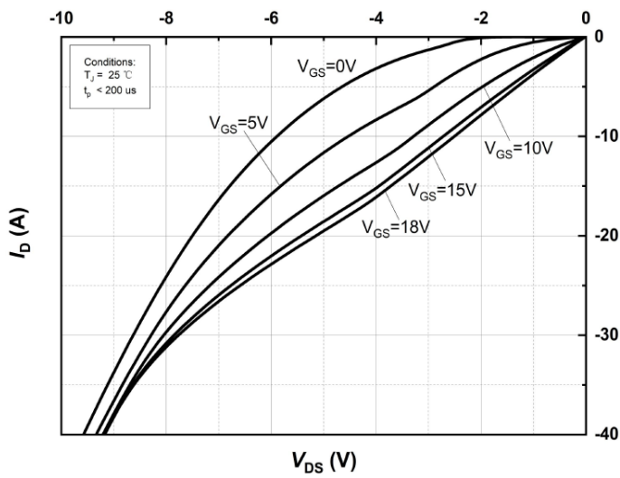
Figure 11. 3rd Quadrant Characteristic at T_J=25^\circ \text{ C}
