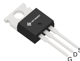
TO-220
