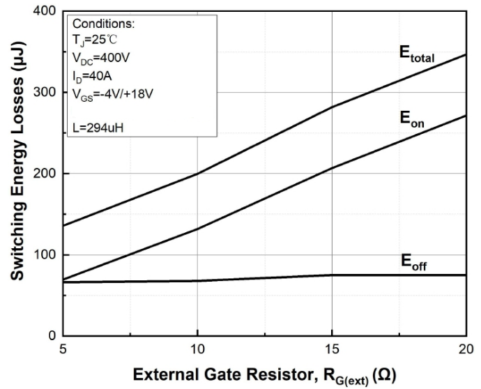
Figure 20. Clamped Inductive Switching Energy vs. R_{G(ext)}
