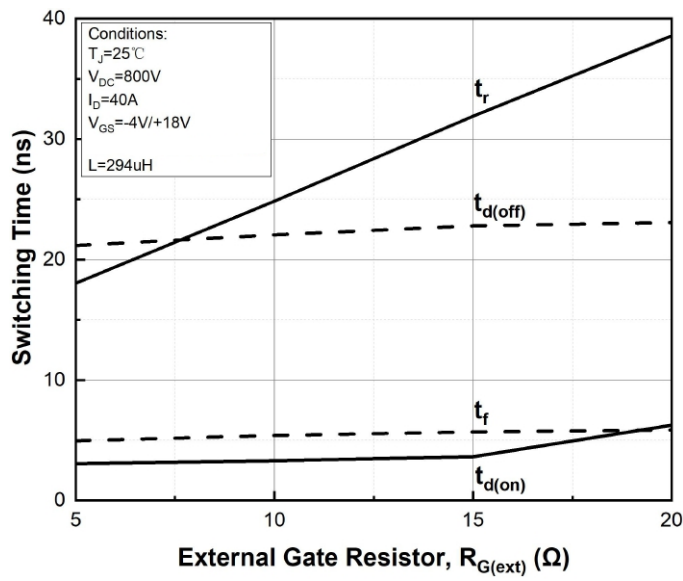
Figure 21. Switching Times vs. R_{G(\text{ext})}
