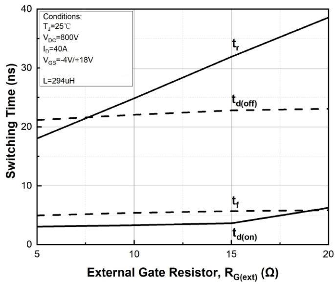
Figure 21. Switching Times vs. R_{G(ext)}
