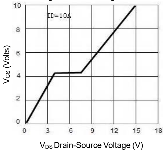
Figure7. Gate Charge
