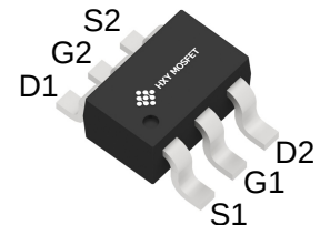
SOT-363 (SOT-363-6)
