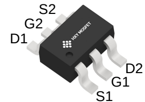
SOT-363 (SOT-363-6)
