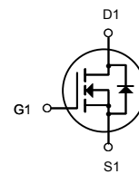
N-Channel MOSFET
