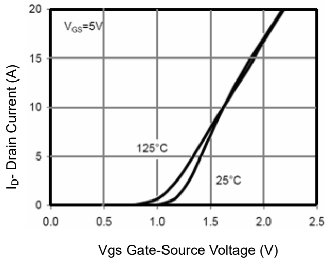
Figure 7 Transfer Characteristics
