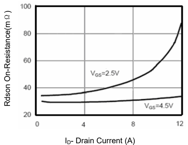
Figure 6 Drain-Source On-Resistance
