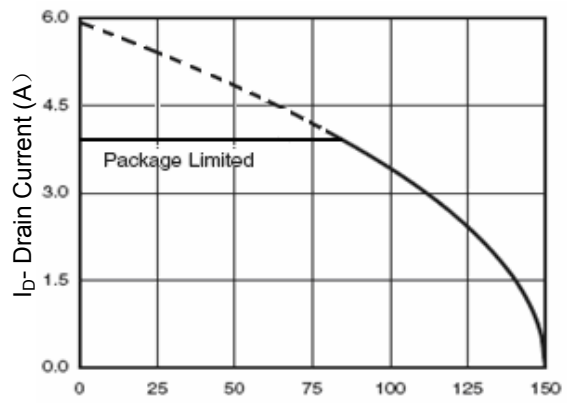
Figure 4 Drain Current
