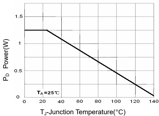
Figure 3 Power Dissipation
