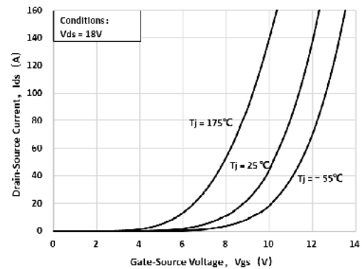
Fig 6: Transfer Characteristic
