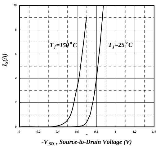
Reverse Diode
