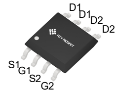
SOP-8 (SOP-8-4.4mm)
