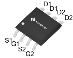
SOP-8 (SOP-8-4.4mm)
