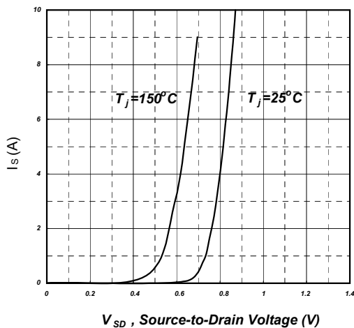
Fig 5. Reverse Diode
