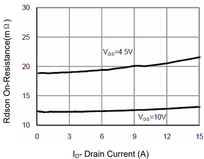
Figure 5 Drain-Source On-Resistance
