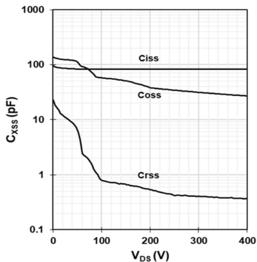
Figure 9 Typ. capacitances
