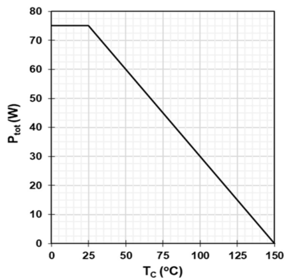
Figure 16 Power dissipation
