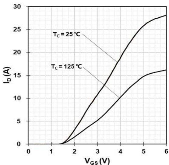
Figure 7 Typ. transfer characteristics
