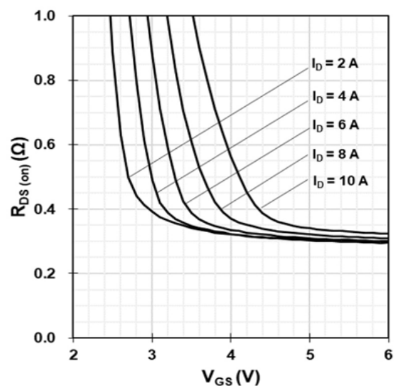
Figure 4 Typ. drain-source on-state resistance
