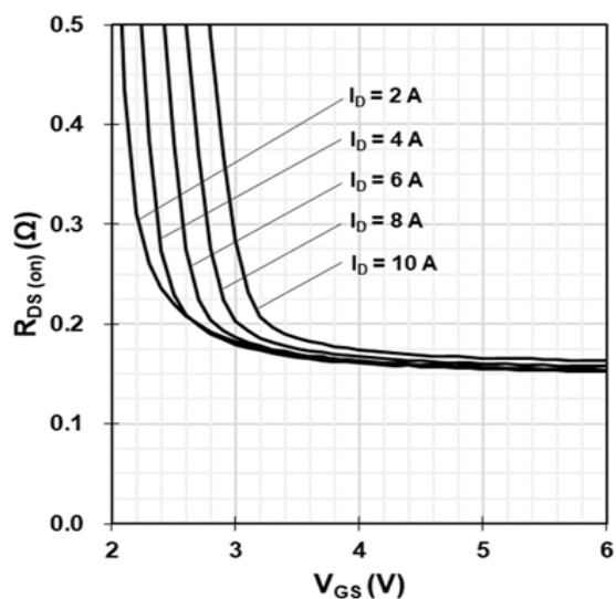
Figure 3 Typ. drain-source on-state resistance
