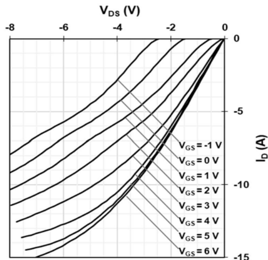
Figure 6 Typ. channel reverse characteristics
