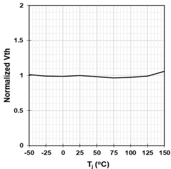
Figure 13 Gate threshold voltage
