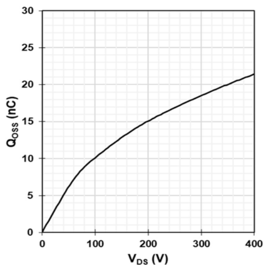
Figure 11 Typ. output charge
