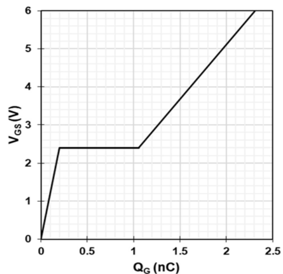
Figure 10 Typ. gate charge
