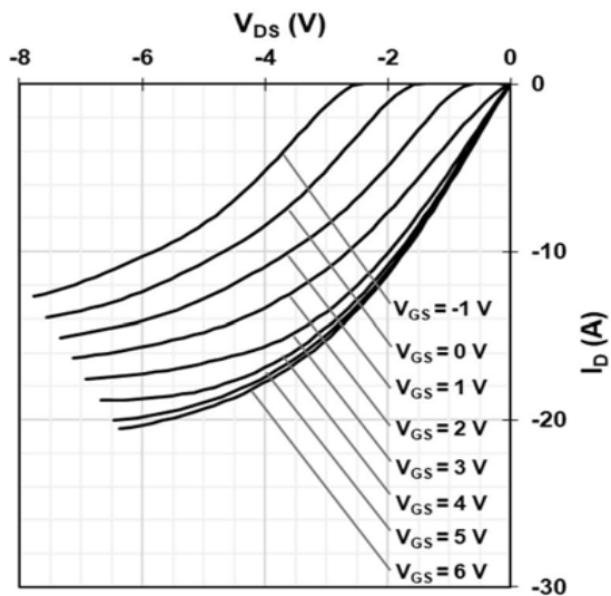
Figure 5 Typ. channel reverse characteristics
