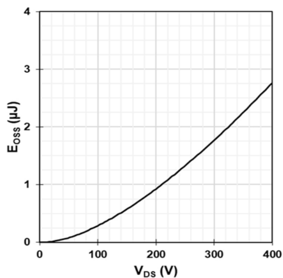
Figure 12 Typ. C oss stored energy
