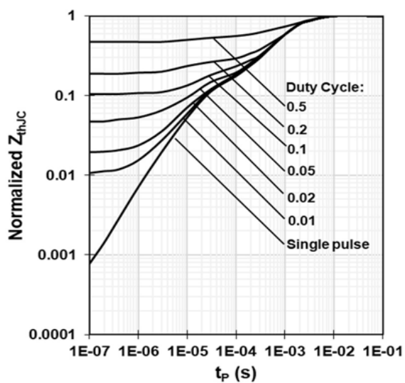
Figure 15 Max. transient thermal impedance
