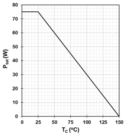
Figure 16 Power dissipation
