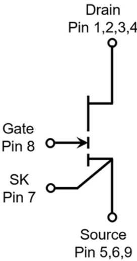
DFN8X8 (DFN-8(8X8))
