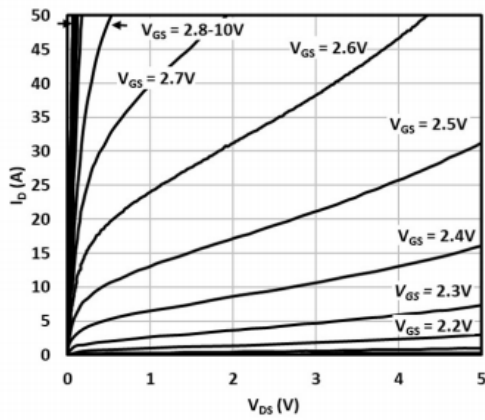
Fig. 1 Output characteristics
