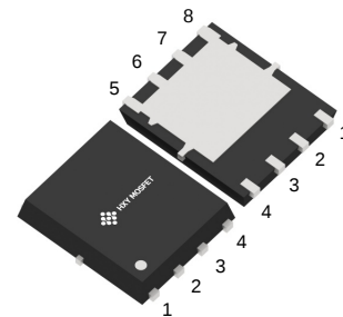
DFN5X6-8L
