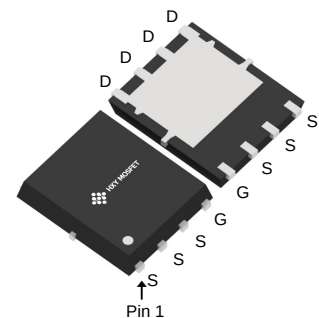
DFN5X6-8L (PDFN-8(5x6))
