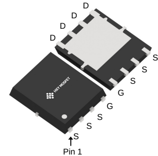
DFN5X6-8L (PDFN-8(5.2x6.2))
