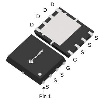
DFN5X6-8L (PDFN-8(5x6))
