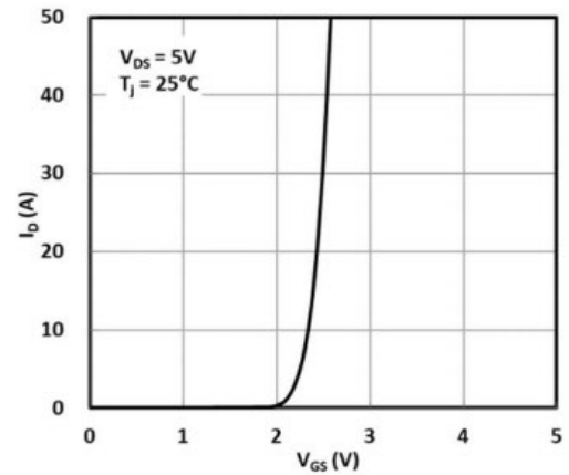
Fig. 2 Transfer characteristics
