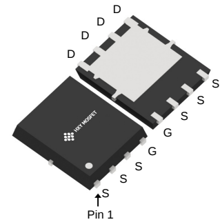
DFN5X6-8L (SO-8-FL-5.8mm)
