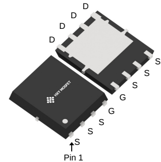
DFN5X6-8L (HSO8)
