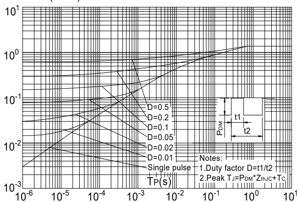
Figure.11: Maximum Effective Transient Thermal Impedance, Junction-to-Case ZthJ-C(°C/W)
