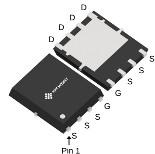
DFN5X6-8L (HSO8-8)
