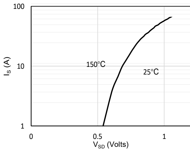
Figure 5: Body-Diode Characteristics
