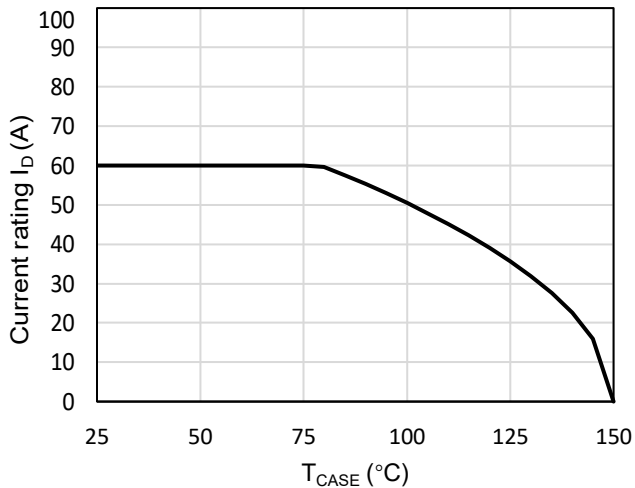
Figure 9: Current De-rating
