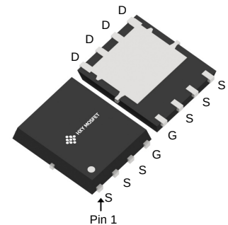
DFN5X6-8L (Power(5x6))
