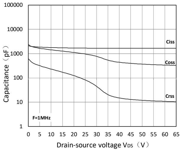
Figure 7. Capacitance Characteristics
