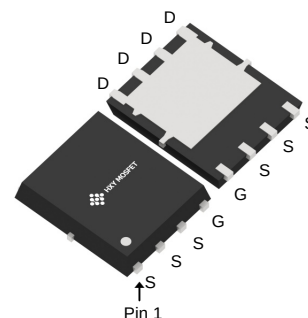
DFN5X6-8L (TDSO-8)
