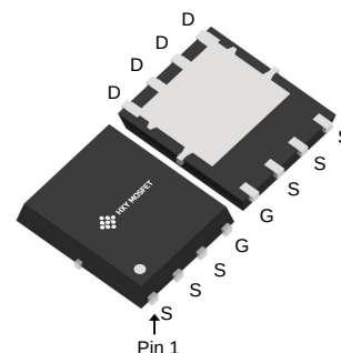
DFN5X6-8L (TDSO-8(5.9x5.2))
