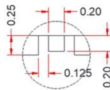
LEAD DETAIL
