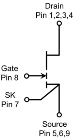
DFN5X6E-8L
