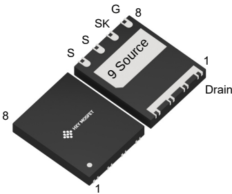
DFN5X6E-8L
