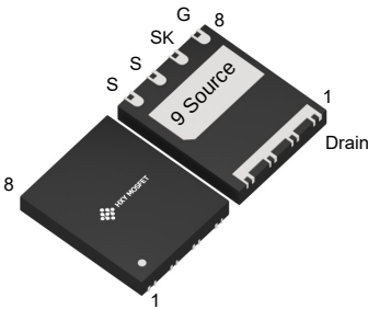
DFN5X6E-8L (DFN-8L(5X6))
