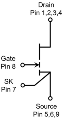
DFN5X6E-8L (DFN-8L(5X6))
