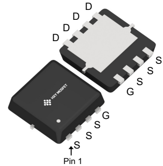
DFN3X3-8L (WDFN-8(3.3x3.3))
