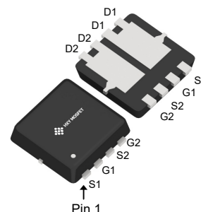
DFN3X3B-8L
